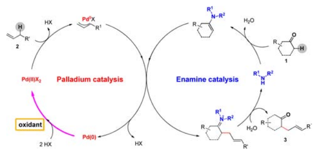
Scheme 2. Mechanistical Assumption for the Oxidative Cross-Coupling between Allylic Hydrocarbons and Unactivated Ketones
